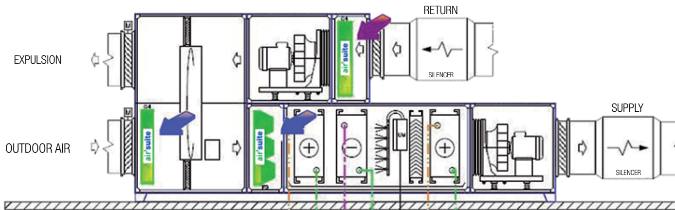
Example of Air'Suite application
