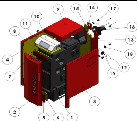
Kotao sa oplatom BIOMAX 23.2 & BIOMAX 35.1 / Boiler of out side jacket BIOMAX 23.2 & BIOMAX 35.1
